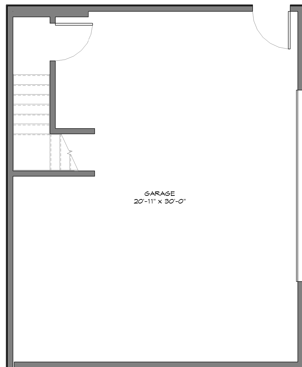
GARAGE FLOOR
