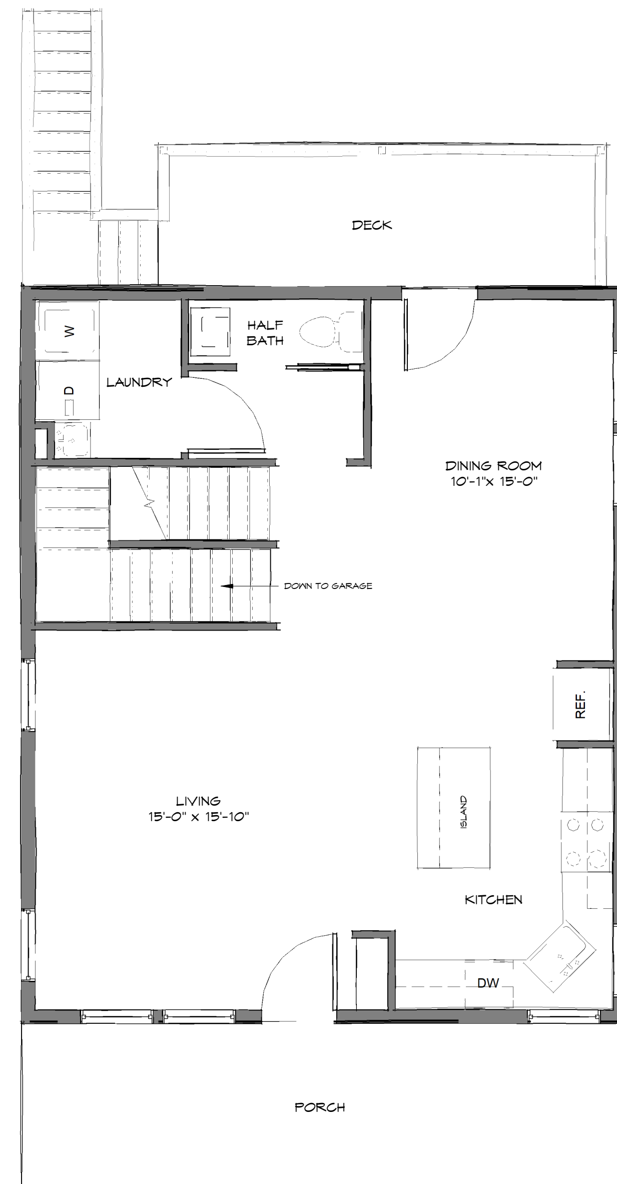
FIRST FLOOR
