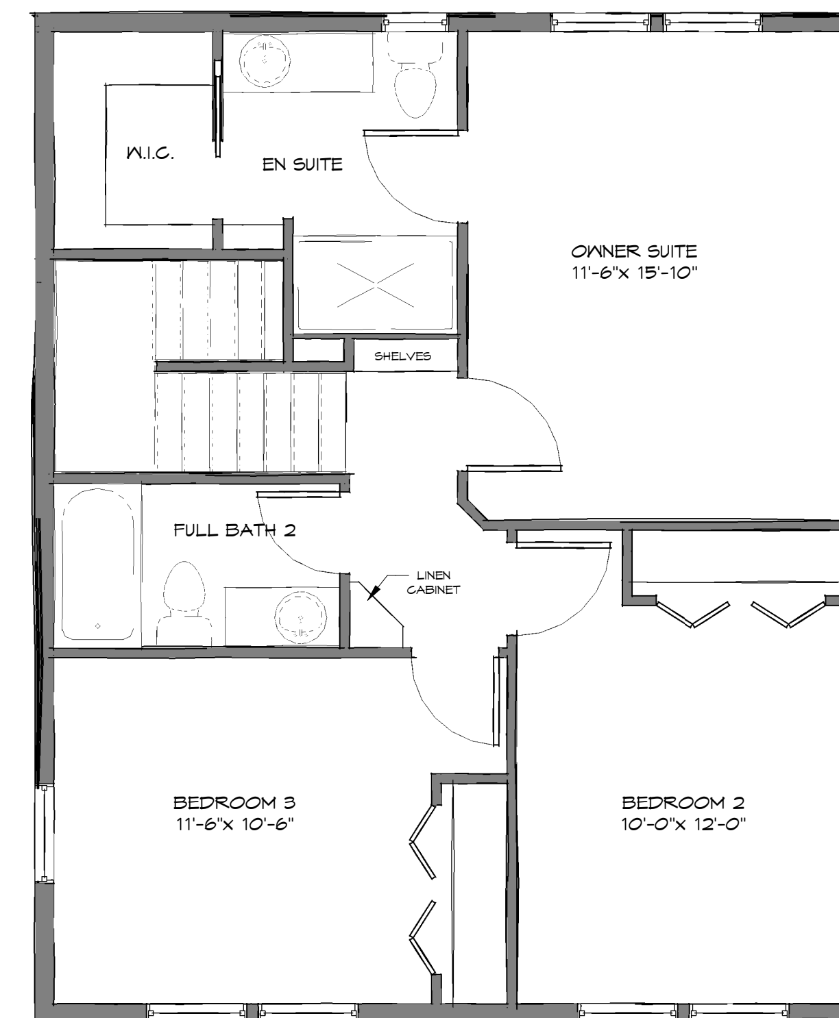
SECOND FLOOR
