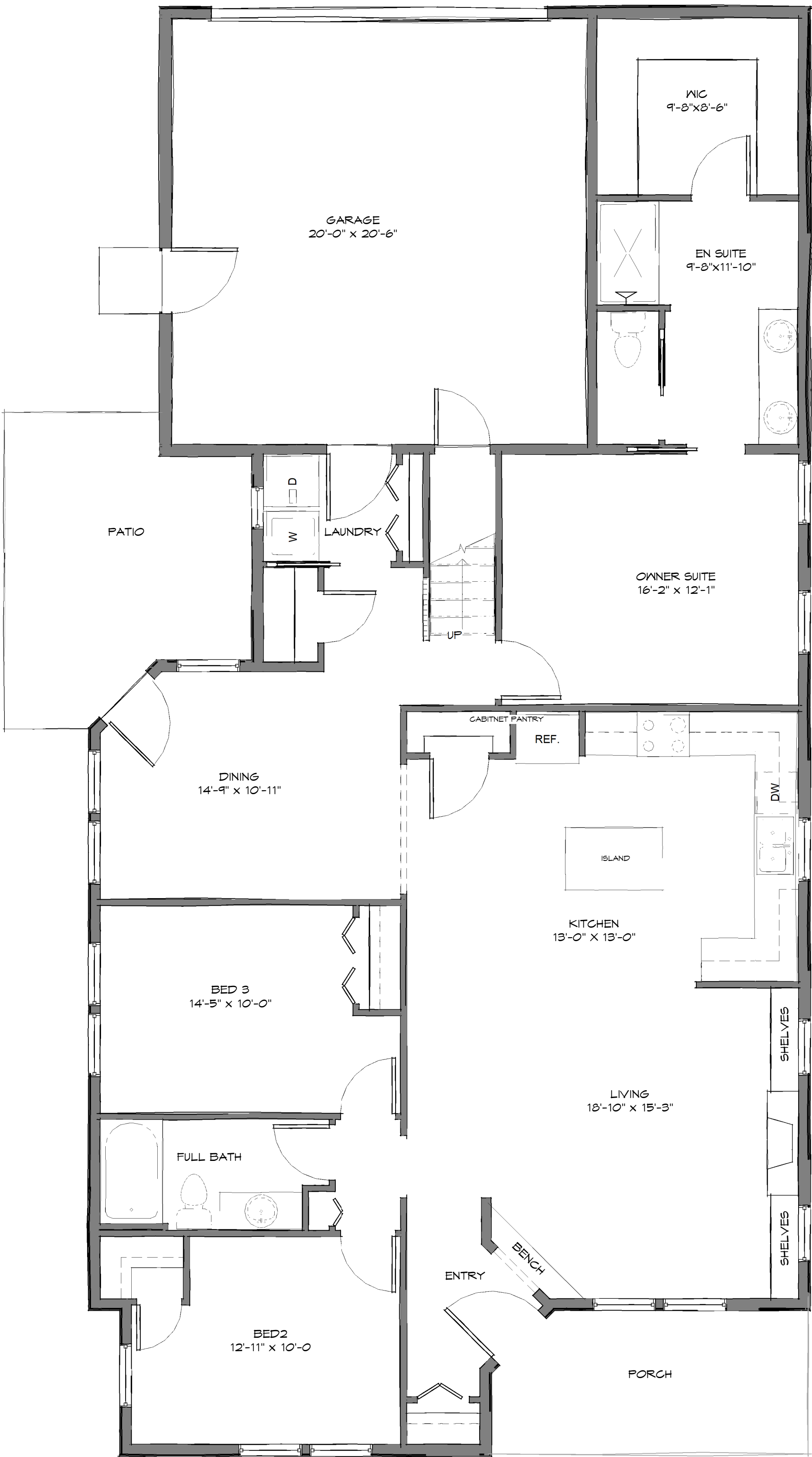
FIRST FLOOR
