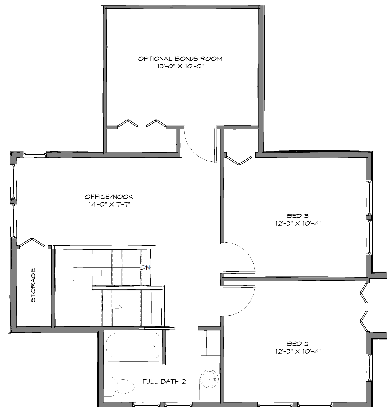
SECOND FLOOR
