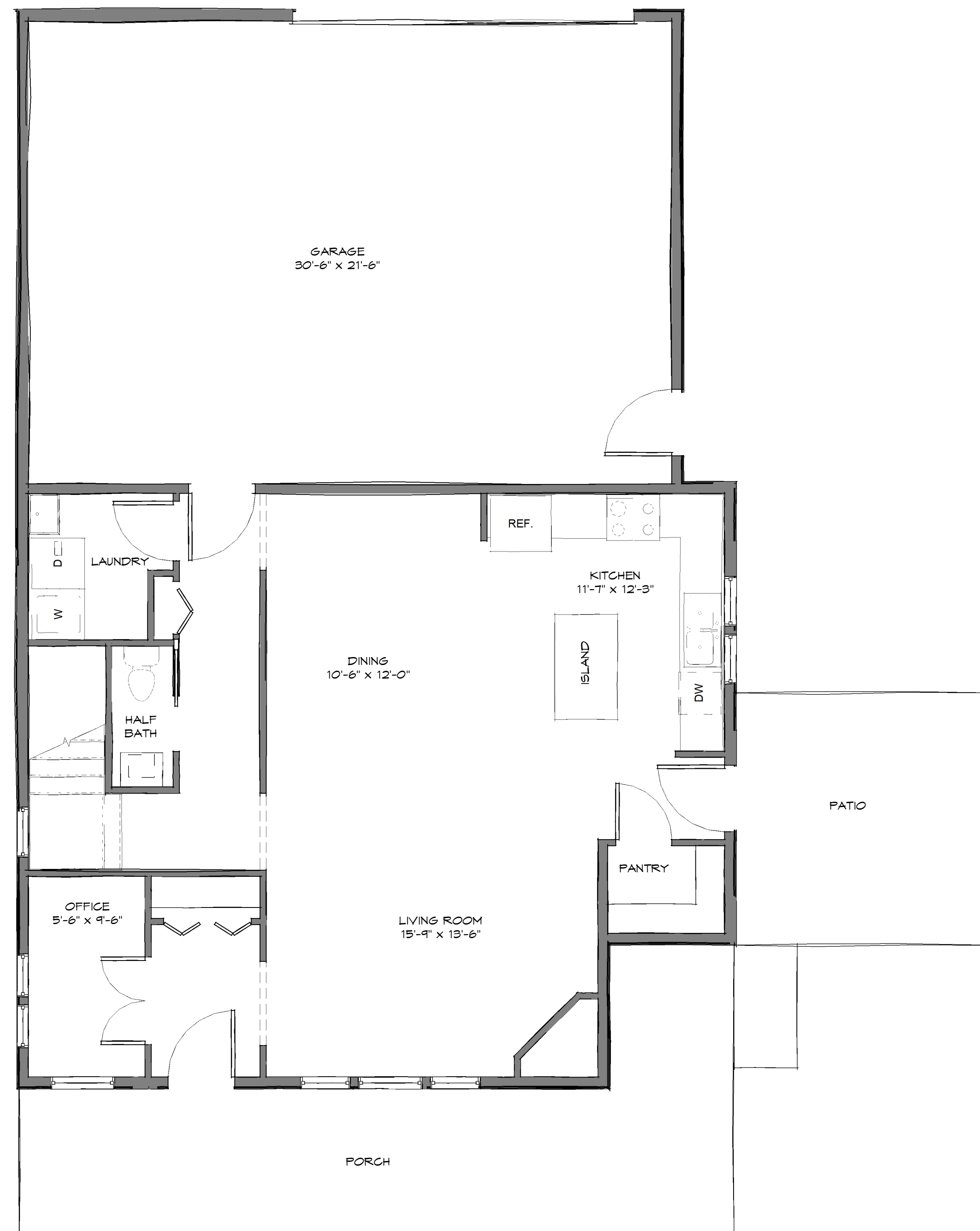
FIRST FLOOR
